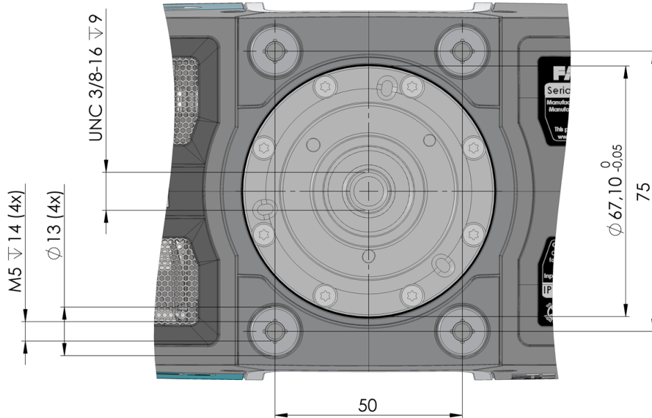
Figure 9-2 Scanner mount
